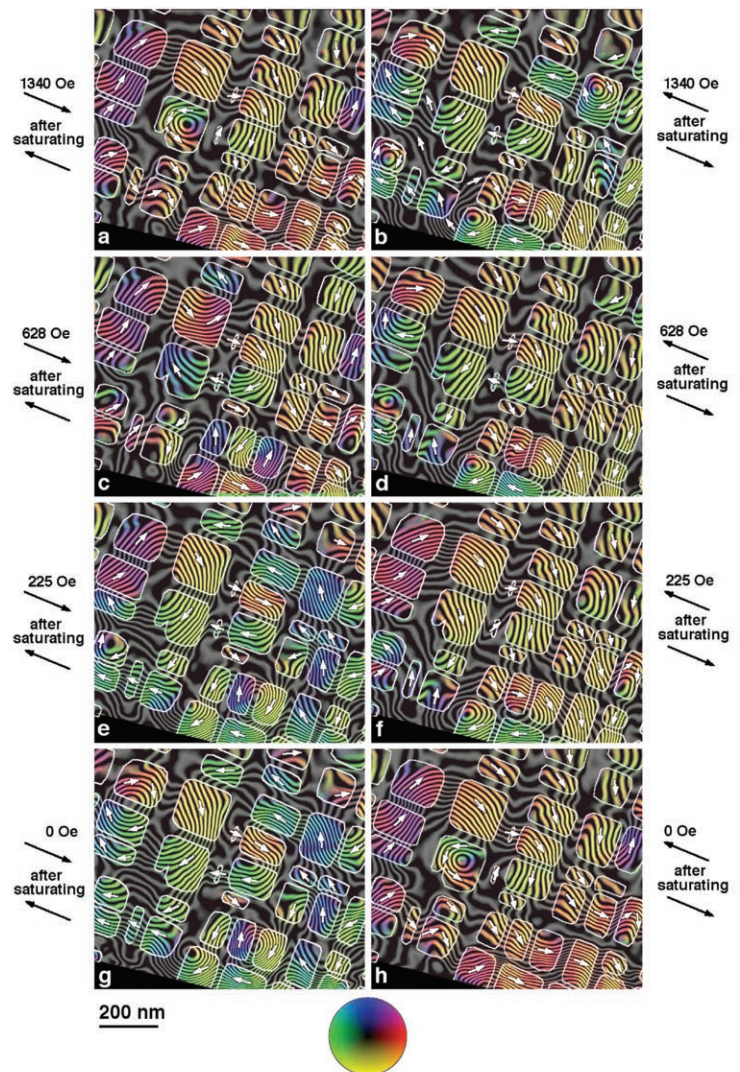
FIGURE 7 Magnetic phase contours from the region shown in Figure 6, measured using electron holography. The outlines of the magnetite-rich regions are marked in white, while the direction of the measured magnetic induction is indicated both using arrows and according to the color wheel shown at the bottom of the figure (red = right, yellow = down, green = left, blue = up). A, C, E, G: obtained after applying a large (1 T) magnetic field towards the top left, then the indicated field towards the bottom right (Oe = oersted). B, D, F, H: obtained after applying identical fields in the opposite directions.
